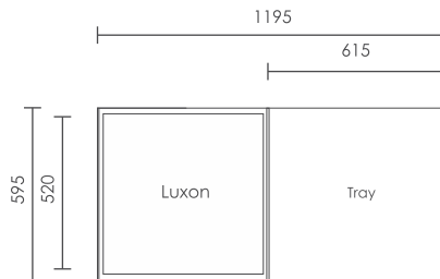
ACCESSORY Offset Ceiling Tray to fit in filed ceiling 600 x 1200mm
