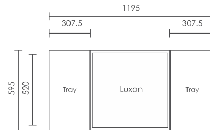
ACCESSORY Side Ceiling Trays to fit in filed ceiling 600 x 1200mm
